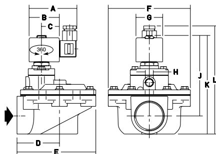
Abb. 1: Gewindeanschlüsse - Aluminium
